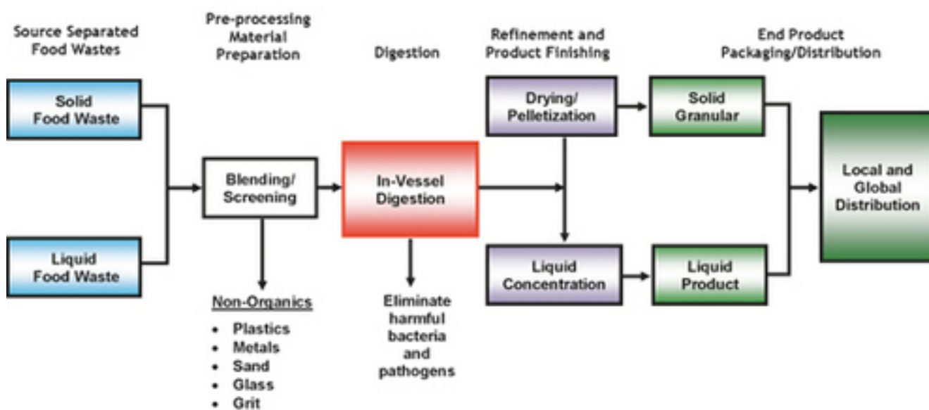
Food Waste Processing Facility Flow Diagram
